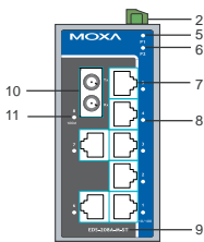
EDS-208A-M-ST Front Panel View
