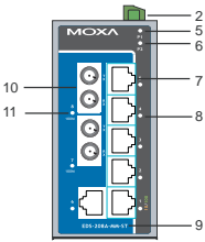
EDS-208A-MM-ST Front Panel View
